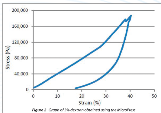
Figure 2 Graph of 3% dextran obtained using the MicroPress
