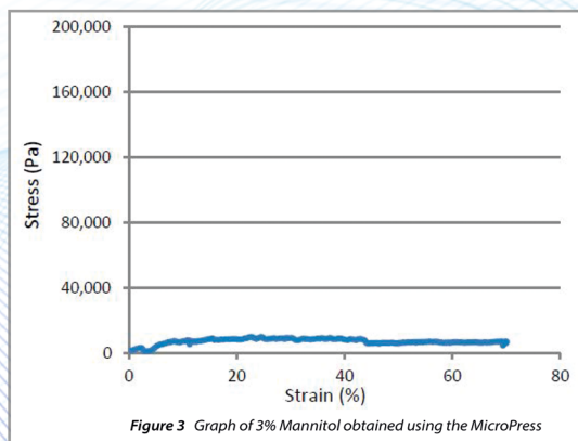
Figure 3 Graph of 3% Mannitol obtained using the MicroPress
